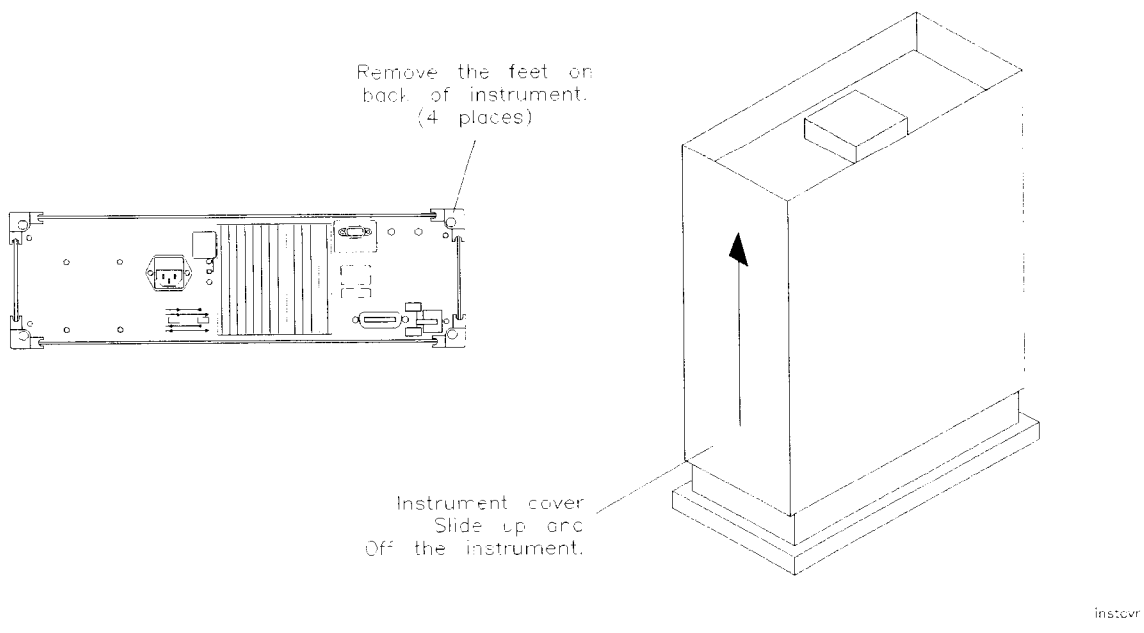
Figure 4-1 Instrument Cover Replacement
