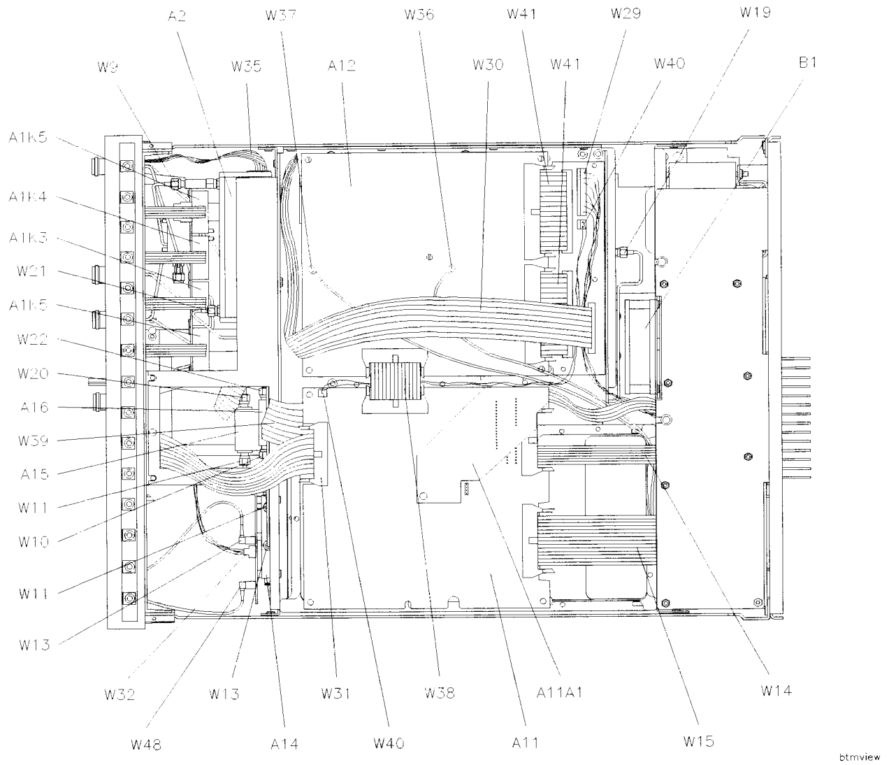
Figure 7-5 Bottom View
