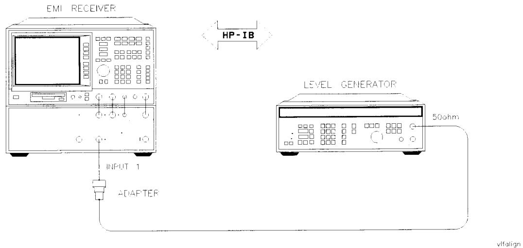
Figure 2-9 Very Low Frequency Alignment, Input 1 Setup
