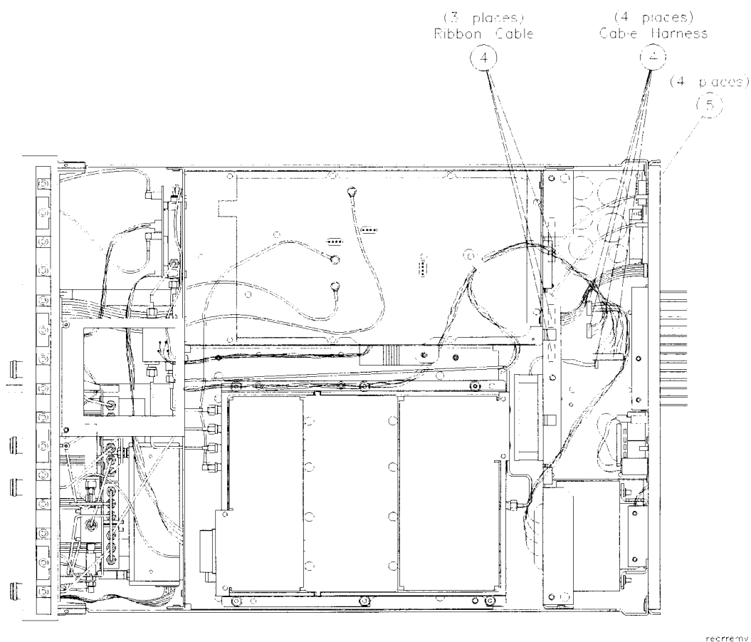
Figure 4-14 Rear-Panel Assembly Replacement, Rear Panel Removal
