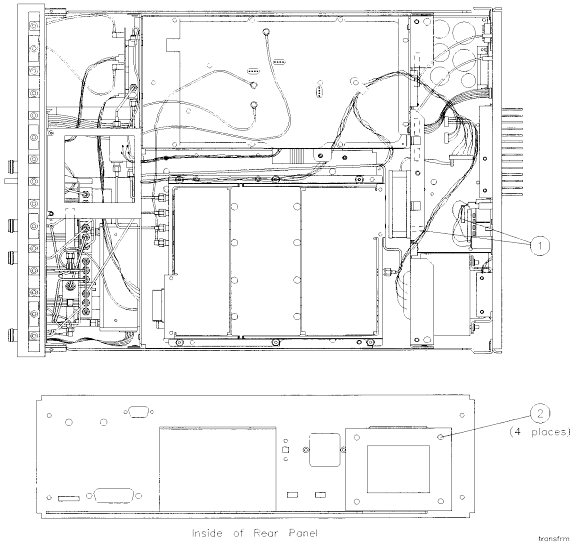
Figure 4-15 T1 Transformer Assembly Replacement
