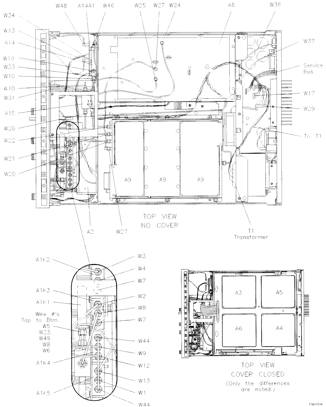
Figure 7-3 Top View
