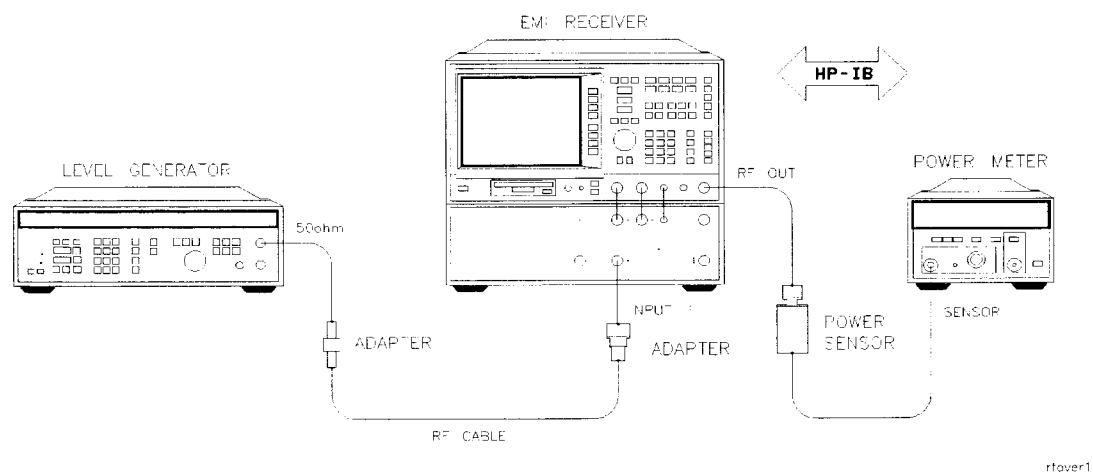
Figure 2-14 RF Overload Calibration, Input 1 Setup
