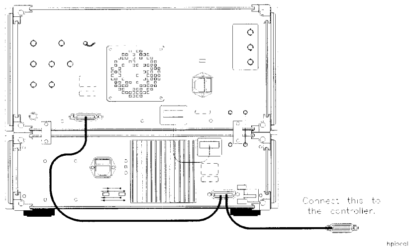
Figure 2-5 RF Filter Section HP-IB Cabling
