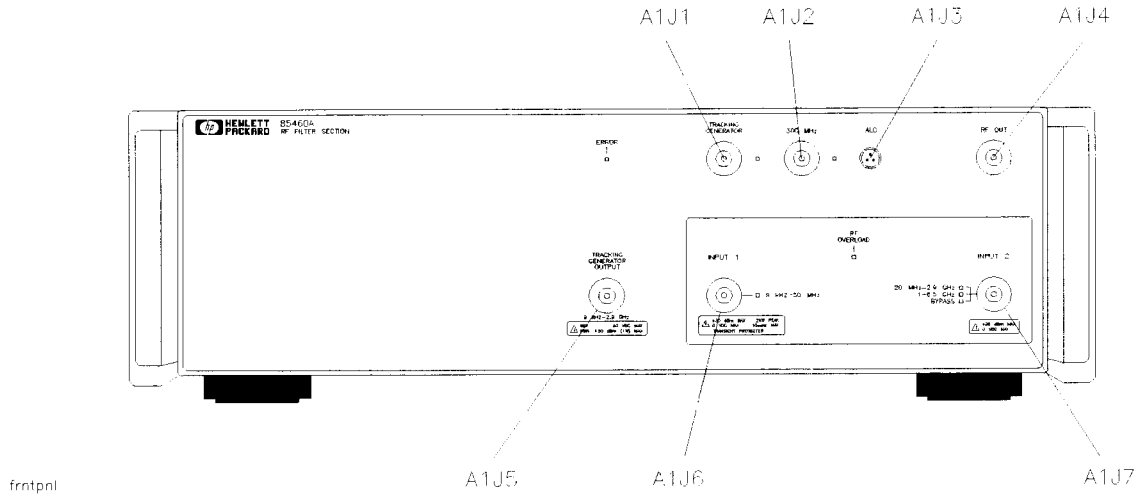
Figure 7-1 Front Panel
