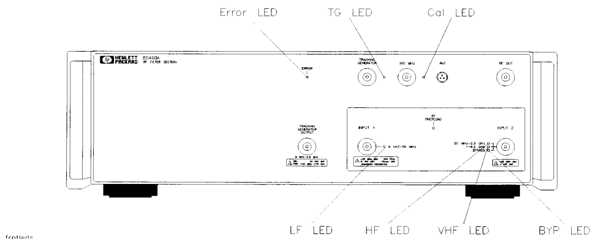
Figure 3-3 Front-Panel LEDs
